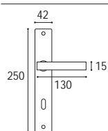
Maniglia con placca rettangolare \text{K} 8 \times 90 Door handle with rectangular plate \text{K} 8 \times 90
