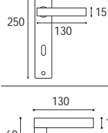
Maniglia con placca rettangolare \text{K} 8 \times 85 yale Door handle with rectangular plate \text{K} 8 \times 85 yale
